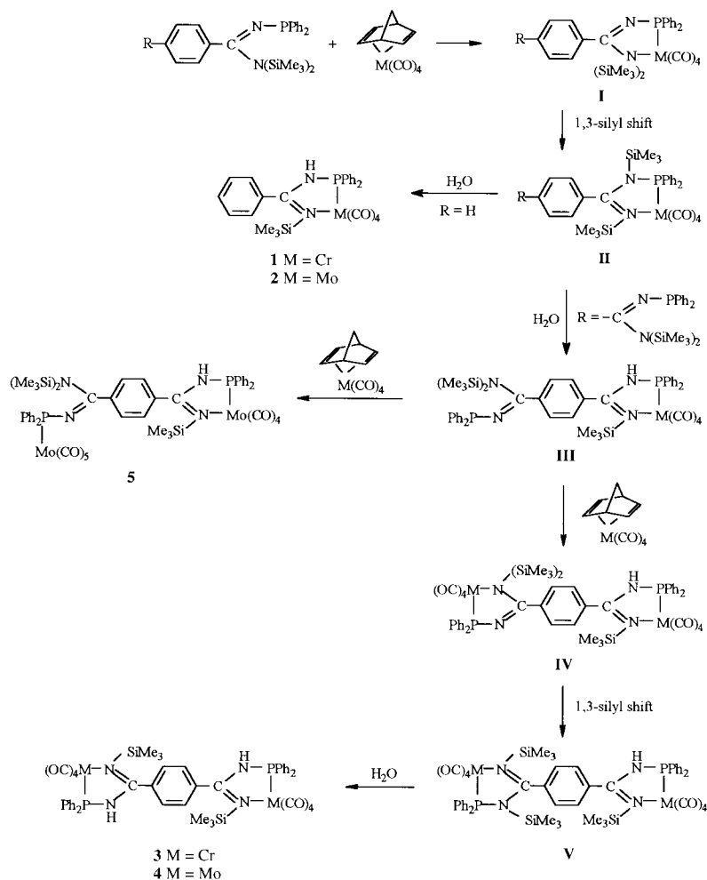
Scheme 1 Possible mechanism for the formation of compounds 1–5
